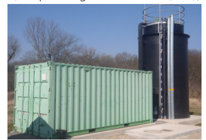
Figure 2: A dosing station (22 m 3 ) and a container with a mixing tank inside.
