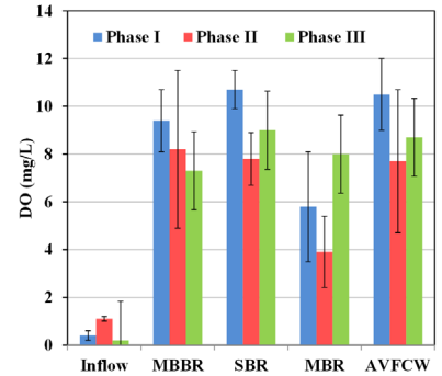
Figure 3: DO concentrations in different experimental phases
