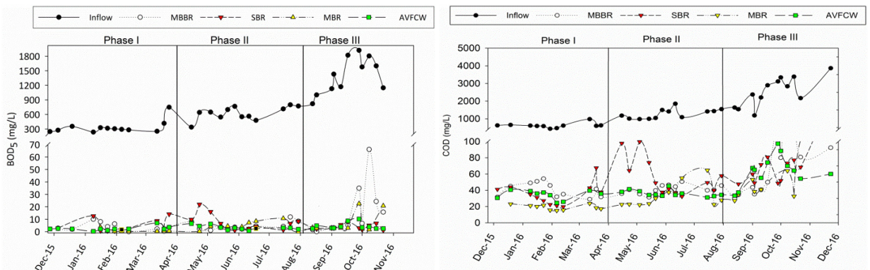
Fig. 4: BOD 5 & COD concentrations
